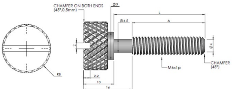
M6 x 40mm Knurled Thumb Screw, Chrome Plated with O-ring, (L)40mm x (A)24mm
