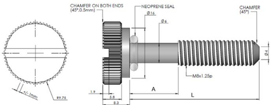
M6 x 30mm Knurled Thumb Screw Chrome Plated with O-ring, (L)30mm x (A)24mm
